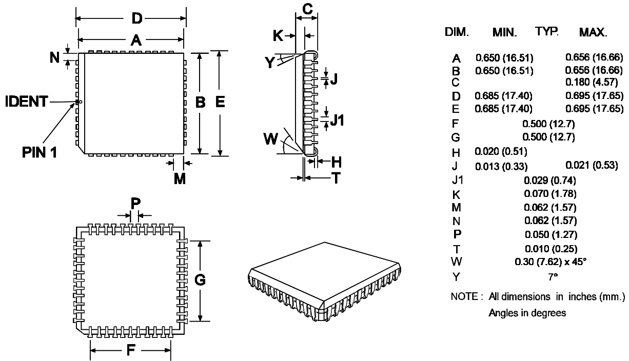
Figure 6 L6 Mechanical Outline: Order as part no. CMX980AL6
